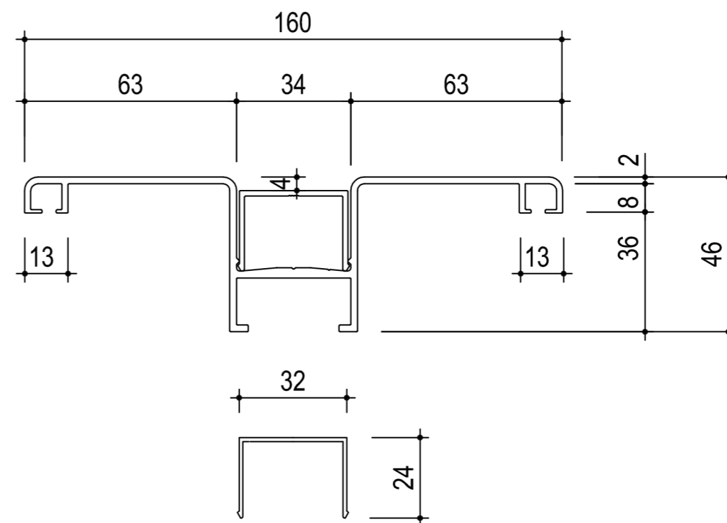
Pilaster strip 160 + covering cap big
