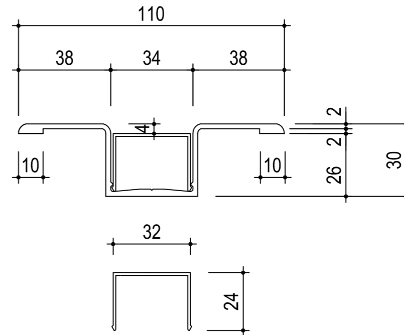
Pilaster strip 110 + covering cap big
