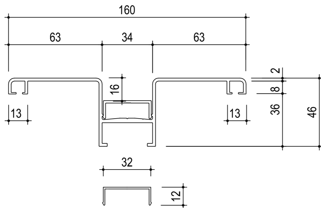
Pilaster strip 160 + covering cap small
