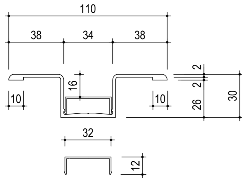
Pilaster strip 110 + covering cap small
