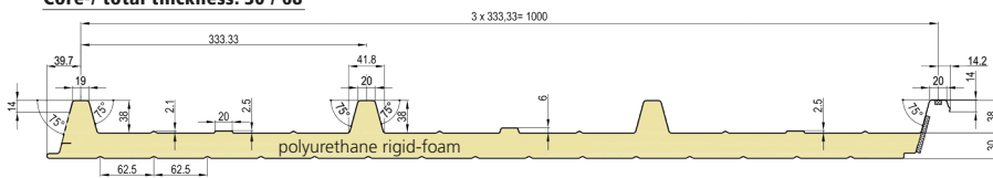
Trapezoidal profile A38-333
